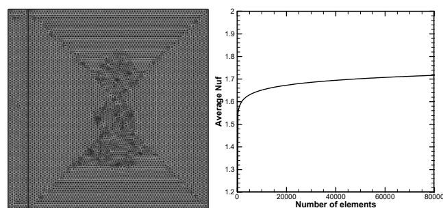
Fig. 2 Two dimensional computational domain within the triangle meshes type (left), the mesh independent study of average Nusselt number (right).
