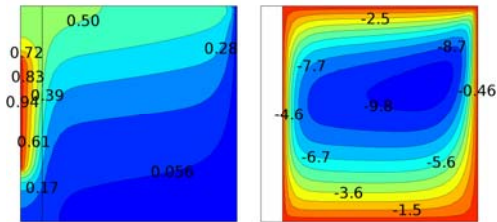
(b) K_r = 1, \overline{Nu}_f = 3.3715, \overline{Nu}_w = 6.3712
