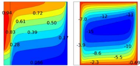
(c) K_r = 10, \overline{Nu}_f = 4.9799, \overline{Nu}_w = 1.7256
