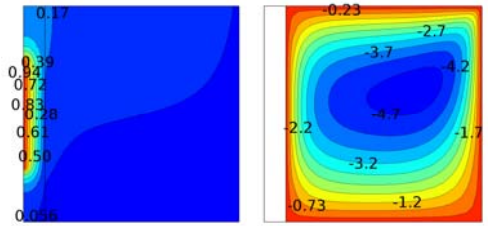
(a) K_r = 0.1, \overline{Nu}_f = 2.8531, \overline{Nu}_w = 9.4808
