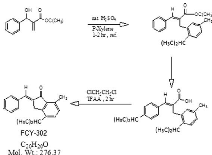
Figure 1. Structure and synthesis of FCY-302.
