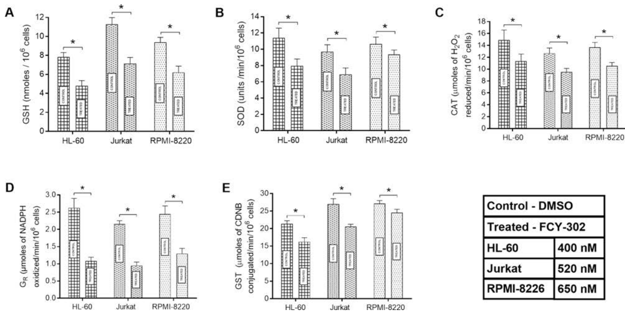
Figure 7. Antioxidant status of FCY-302-treated cancer cells. Levels of (A) GSH, activities of (B) superoxide dismutase (SOD), (C) catalase (CAT), (D) glutathione reductase ( \text{G}_R ), and (E) glutathione-S-transferase (GST) post-FCY-302 treatments. Results are expressed as mean value \pm SD. *p < 0.05 .
