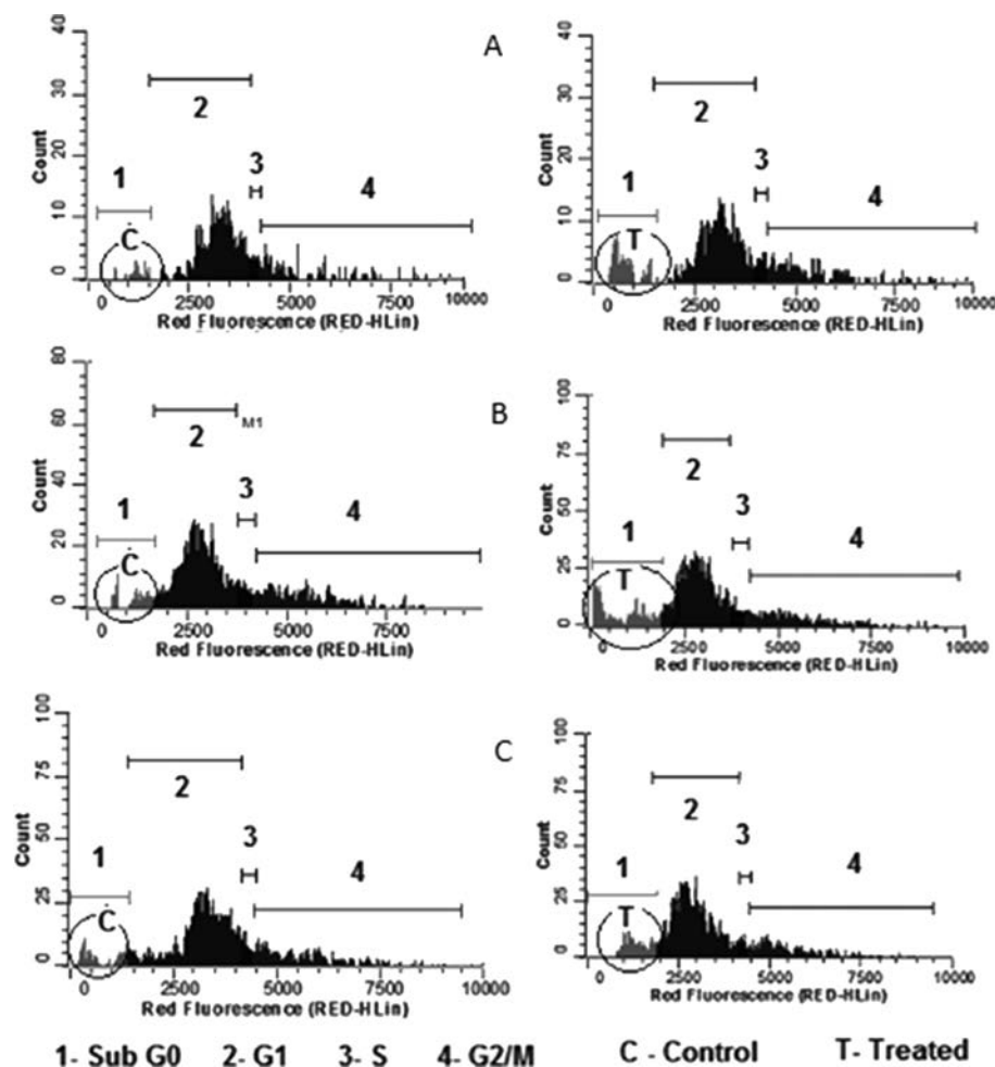
Figure 3. Cell cycle analysis of (A) HL-60, (B) Jurkat, and (C) RPMI-8226 cells after 72 h treatment of FCY-302. Representative cell cycle histograms from three individual experiments showing percentage sub-G 0 population in cancer cells after FCY-302 treatments.
