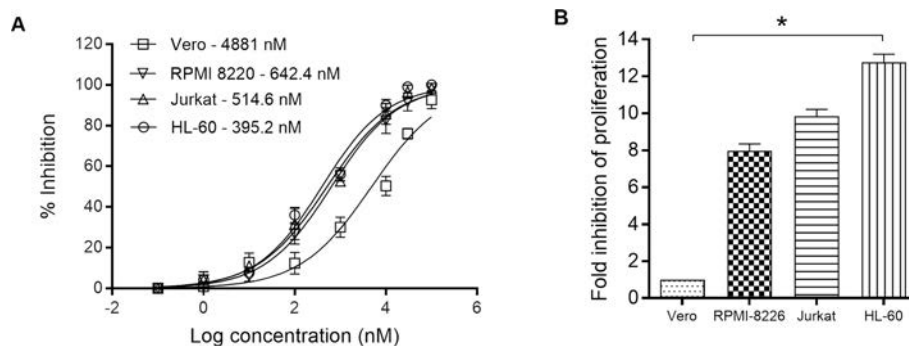
Figure 2. Efficacy of FCY-302 in cancer and normal cells. (A) \text{GI}_{50} values of FCY-302 in HL-60, Jurkat, RPMI-8226, and Vero cells showing antiproliferative effects by 3-(4,5-dimethylthiazol-2-yl)-2,5-diphenyltetrazolium bromide (MTT) assay. (B) Fold difference in antiproliferative efficacy by the compound between normal and cancerous cells. Results are average from three individual experiments performed in triplicates. * p < 0.05 .
