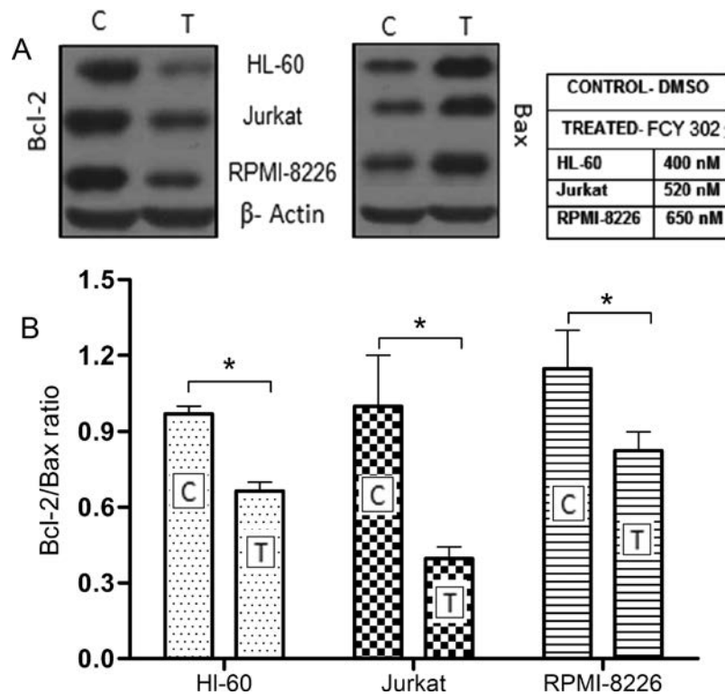
Figure 5. (A) Western blot of antiapoptotic and proapoptotic markers after various doses of FCY-302 treatment in HL-60, Jurkat, and RPMI-8226 cells for 48 h. (B) Bcl-2/Bax ratio of HL-60, Jurkat, and RPMI-8226 cells after FCY-302 treatment. Bands were quantified by densitometry using ImageJ (Ver: 1.46, NIH), normalized to actin, results were plotted with GraphPad Prism 6 software. Results are from three individual experiments in duplicates and were statistically significant at *p < 0.5 .
