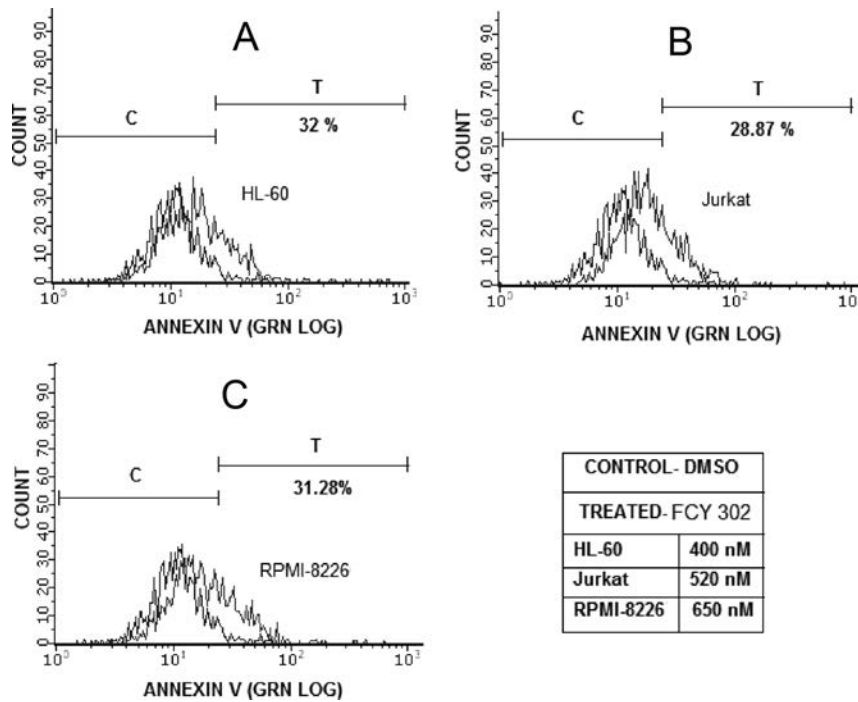
Figure 4. Representative histograms from annexin V assay post-FCY-302 treatment in (A) HL-60, (B) Jurkat, and (C) RPMI-8226 cells after 48 h. Results from three independent assays are shown.
