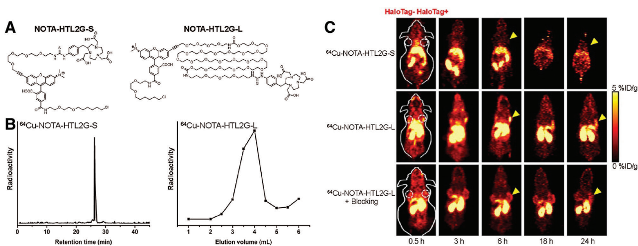
FIGURE 5. (A) Chemical structures of NOTA-HTL2G-S and NOTA-HTL2G-L. (B) HPLC of ^{64}Cu -NOTA-HTL2G-S and size exclusion chromatography of ^{64}Cu -NOTA-HTL2G-L. (C) Serial PET images of mice bearing both 4T1 (left) and 4T1-HaloTag-ECS (right) tumors at different time points post-injection of ^{64}Cu -NOTA-HTL2G-S, ^{64}Cu -NOTA-HTL2G-L, or ^{64}Cu -NOTA-HTL2G-L with blockage (N = 4). Reproduced with permission from Hong et al. (2013).
