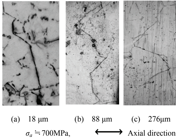
Figure 7: Morphologies of cracks under ultrasonic loading
