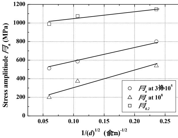
Figure 4: Grain size dependence of fatigue strength
