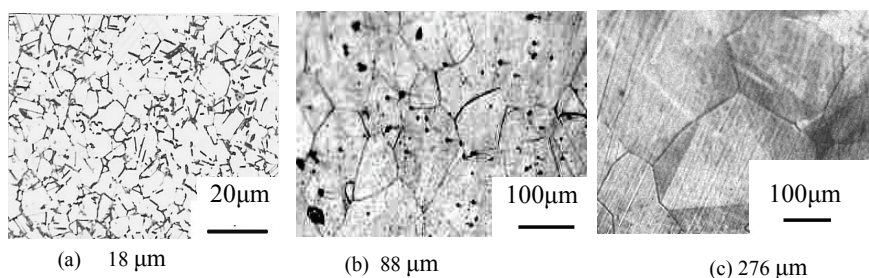
Figure 1: Microstructures of tested alloys
