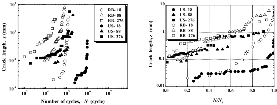
Figure 5: Crack growth curves ( \sigma_a=700\text{MPa} )
