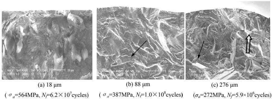
Figure 8: Fracture surfaces under ultrasonic loading
