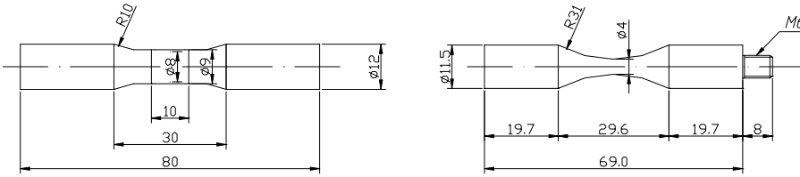
Figure 2: Shape and dimensions of specimens
