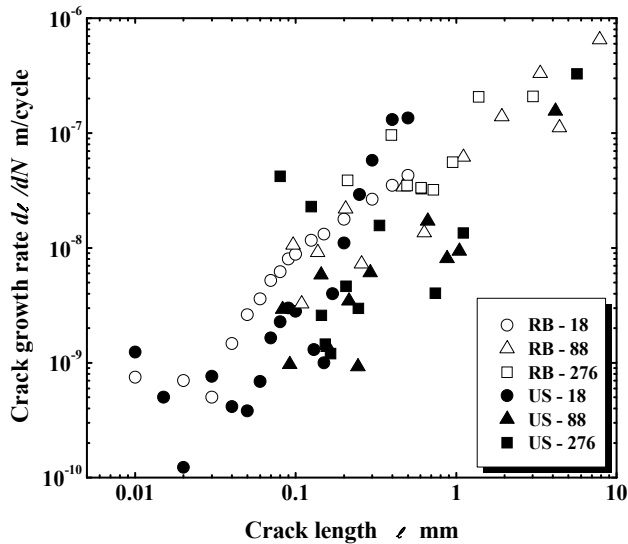
Figure 6: Crack growth rate against for crack length
