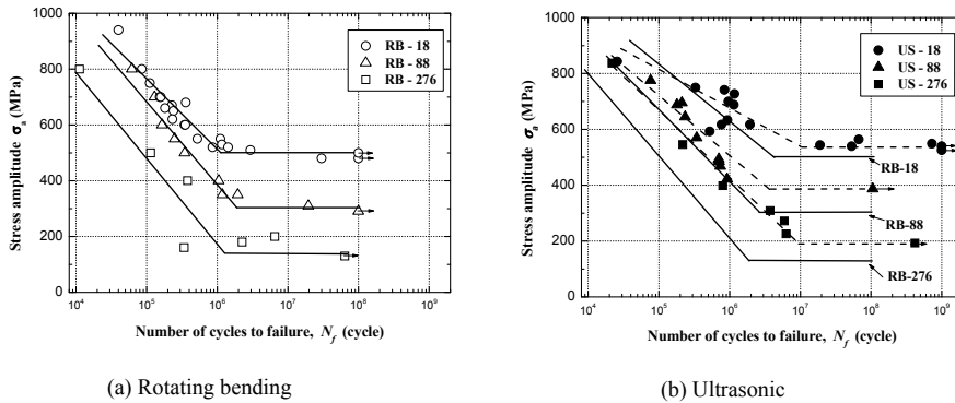
Figure 3: S-N curves
