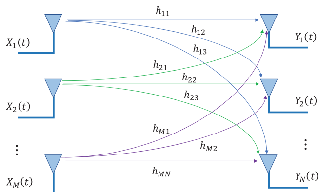
Figure 1: Simplified MIMO channel in terahertz communication
