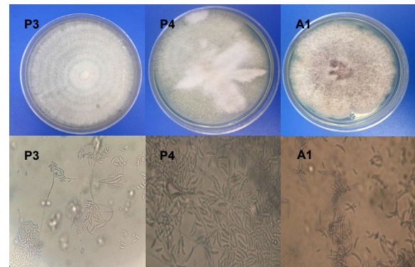
Fig. 1. Macroscopic and microscopic characteristics of Fusarium sp. (P3, P4 and A1).
