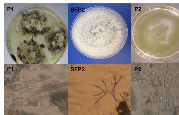
Fig. 2. Macroscopic and microscopic characteristics of Metarrhizium sp. (P1) Nigrospora sp. (SFP2) and Penicillium sp. (P2).
