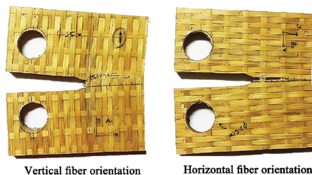
Figure 12: Fiber orientations of bamboo mat plywood [72]
