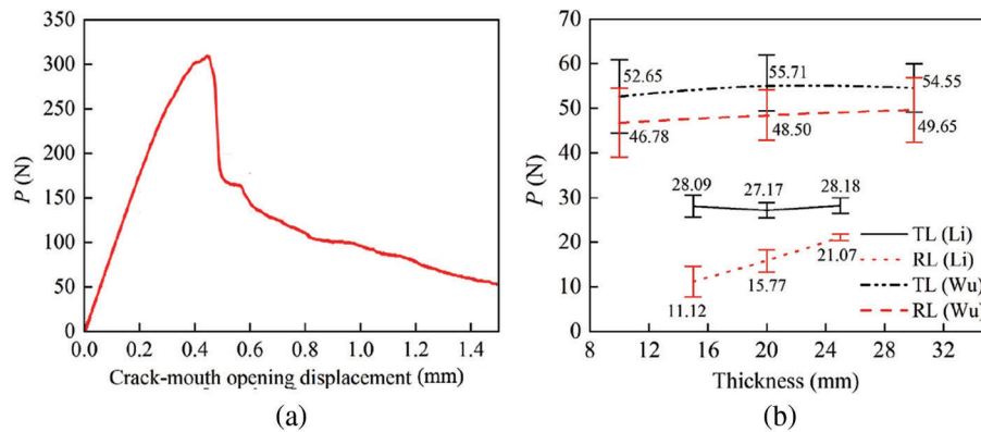
Figure 13: Fracture parameters in the literature [73] and literature [74]: (a) Typical load displacement curve of CT specimen [74]; (b) Comparison of fracture toughness [73,74], where, P is the load; in “TL” and “RL”, the first letter indicates the crack opening direction, and the second letter indicates the crack extension direction
