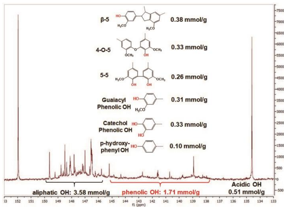
Figure 4 31 P-NMR analysis of Bio-oil.
