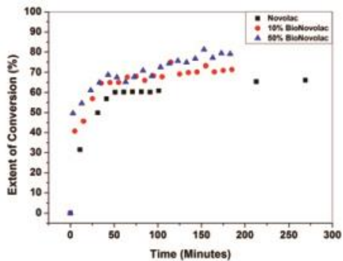
Figure 6 BioNovolac Extent of Conversion (Refer Equation (4)).
