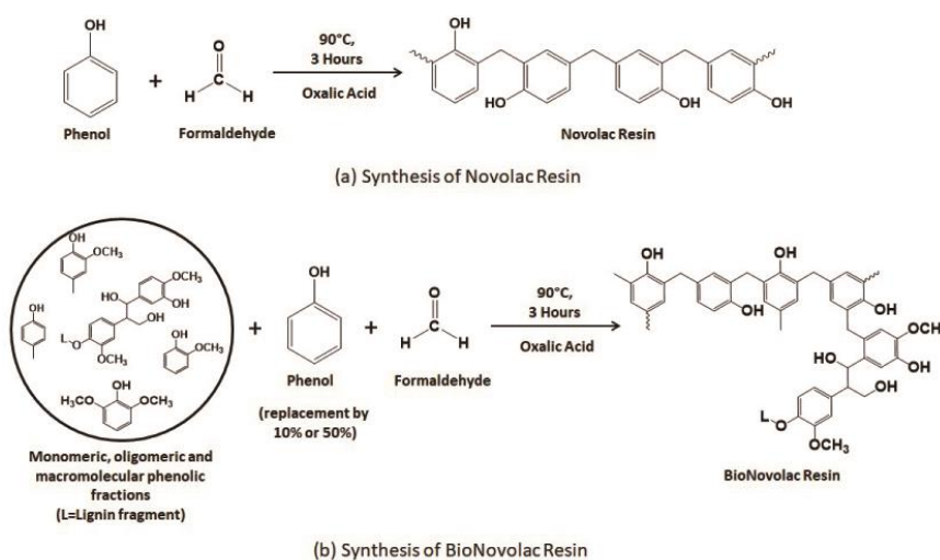
Figure 1 (a) Synthesis of novolac resin, (b) Synthesis of BioNovolac resin.
