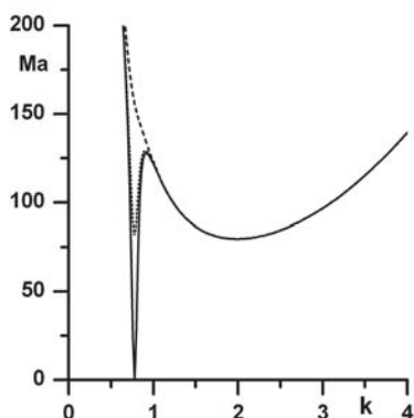
Figure 2: Neutral curves Ma^+(k) for k > 1 (Pearson curve). (a) Cowley-Rosensweig marginal case (solid line), (b) Cowley-Rosensweig stable case showing a finite minima at k \sim O(\sqrt{Bo}) (dotted line), and (c) case when the magnetic field has a negligible influence (dashed line).
