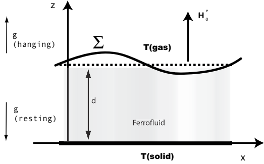
Figure 1: Ferrofluid layer submitted to a normal constant magnetic field \mathbf{H}_0^e = H_0^e \mathbf{1}_z and to a normal temperature gradient \Delta T = T(\text{gas}) - T(\text{solid}) . \mathbf{1}_z = unit normal directed from solid into gas, \mathbf{1}_x = horizontal unit vector along z = 0 .
