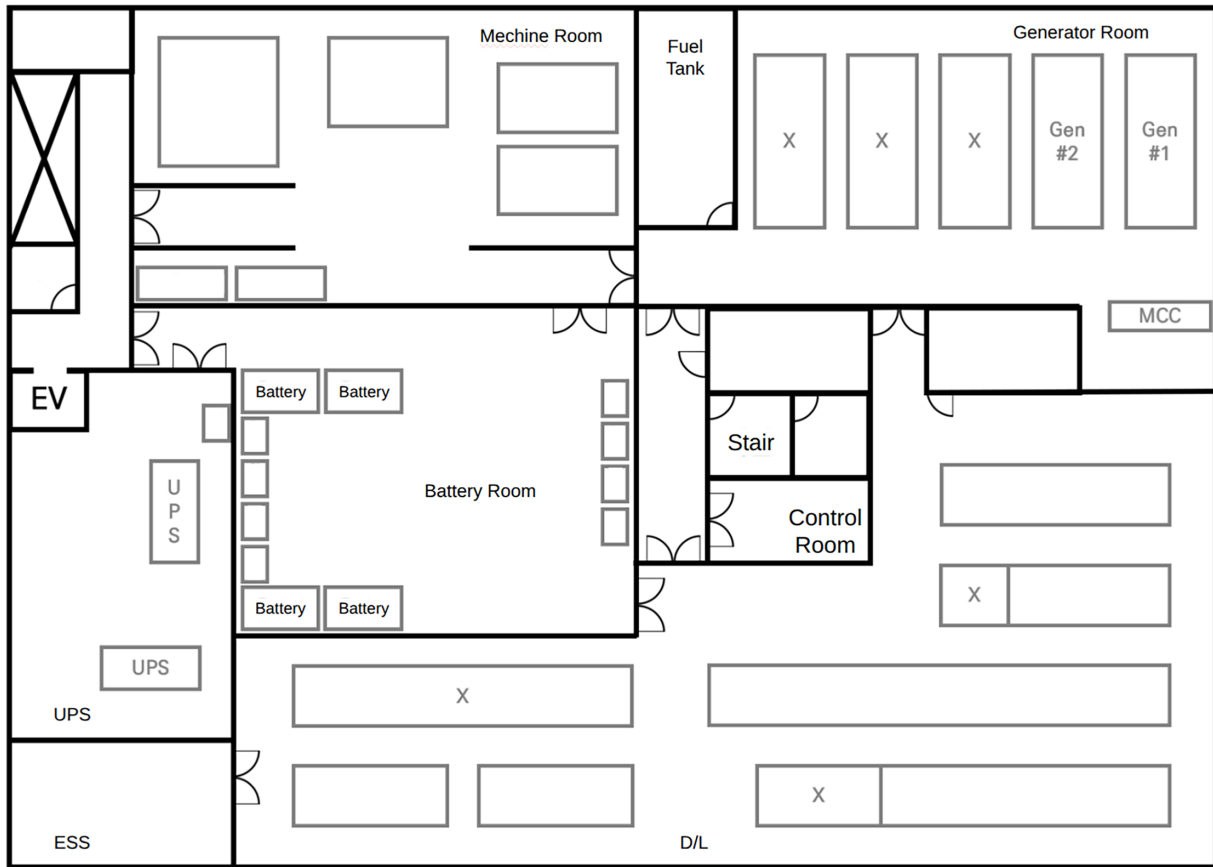
Figure 2: Inspection map of the underground infrastructure of the KEPCO Power ICT Center.
