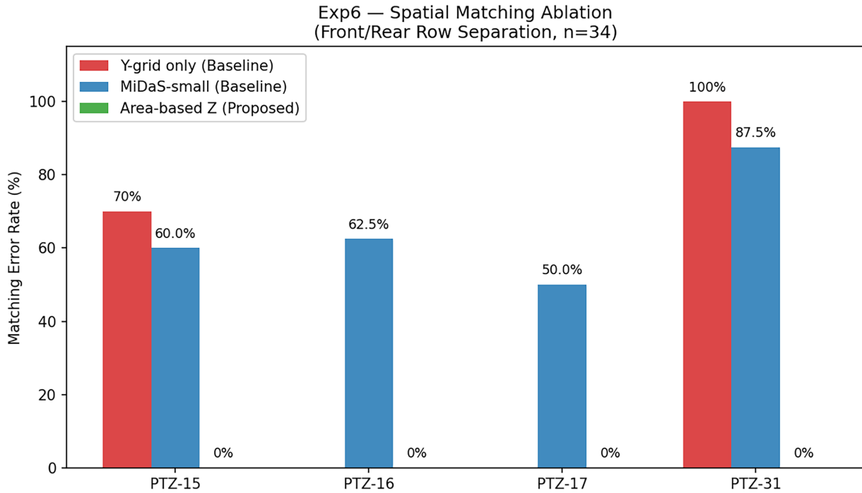
Figure 7: Spatial match error rates by scene ( n = 34 ): Y-axis grid, MiDaS-small, and area-based Z-depth.
