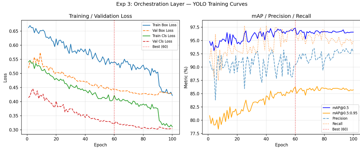
Figure 6: Classifier (YOLO) training curves.
