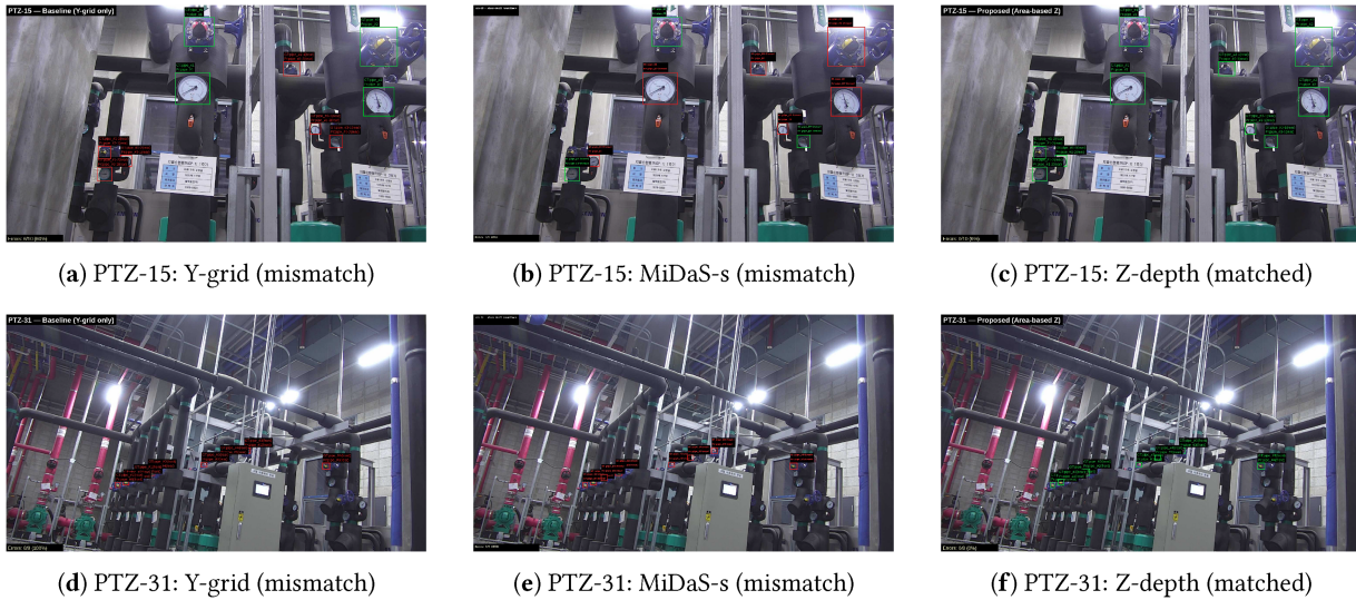
Figure 8: Qualitative comparison of front/rear matching (Y-grid/MiDaS-small/Z-depth).
