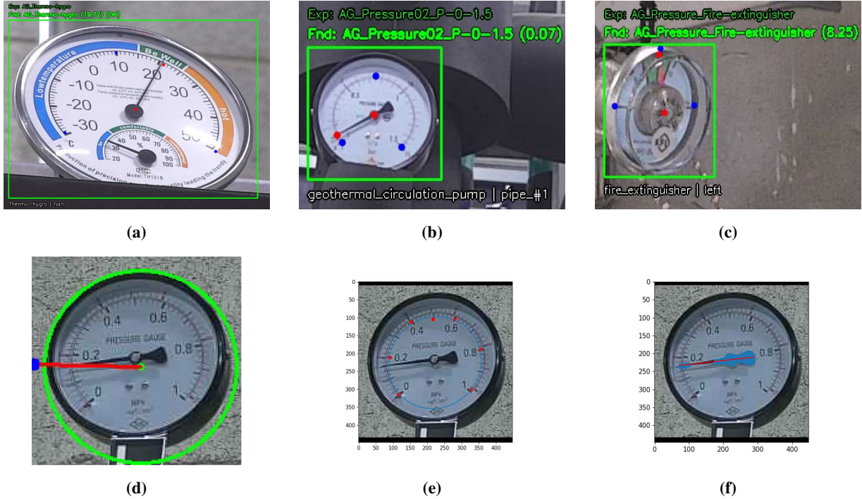
Figure 9: Examples of analog gauge readings and comparison with baselines. (a) Thermometer reading (b) Pressure gauge reading (c) Fire extinguisher pressure gauge (d) Hough-Circle (e) ETH scale keypoints (f) ETH needle segmentation.
