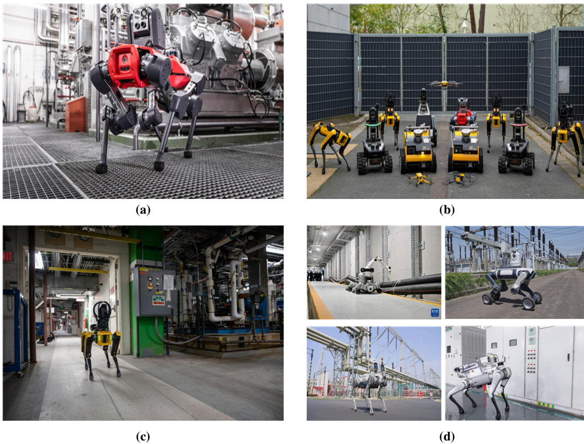
Figure 1: Major industrial quadruped robots. (a) ANYbotics ANYmal (b) Energy Robotics (c) Boston Dynamics Spot (d) Deep Robotics quadruped robot.
