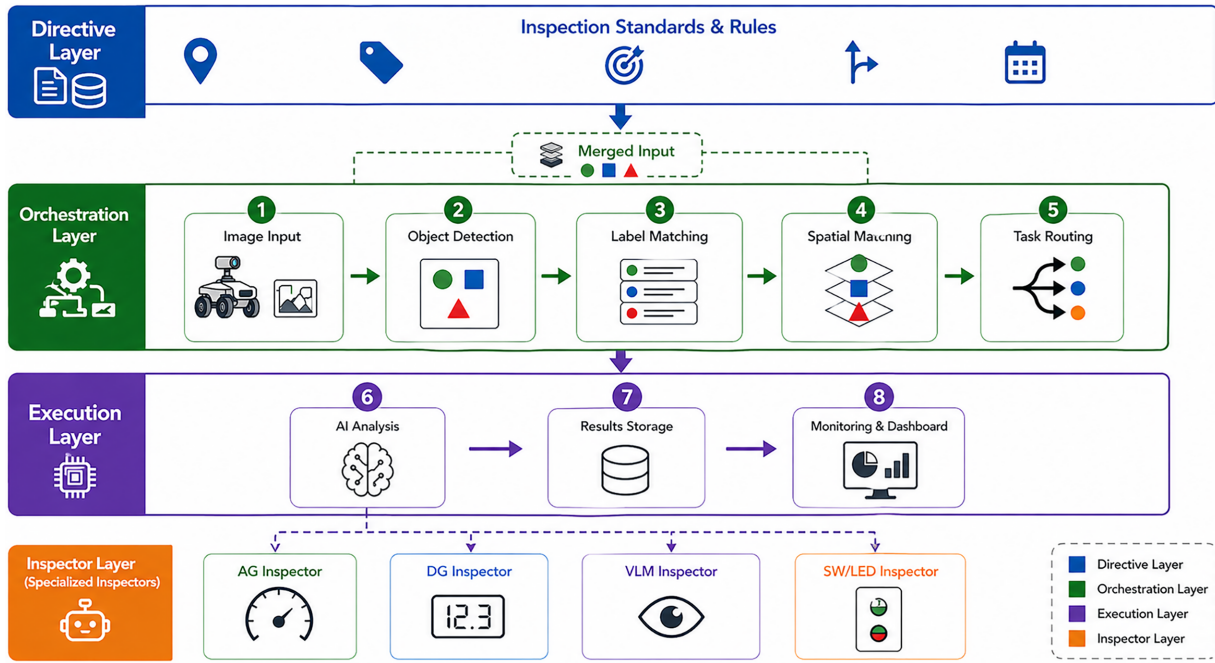
Figure 5: Overall flow of the AI inspection and diagnosis pipeline.
