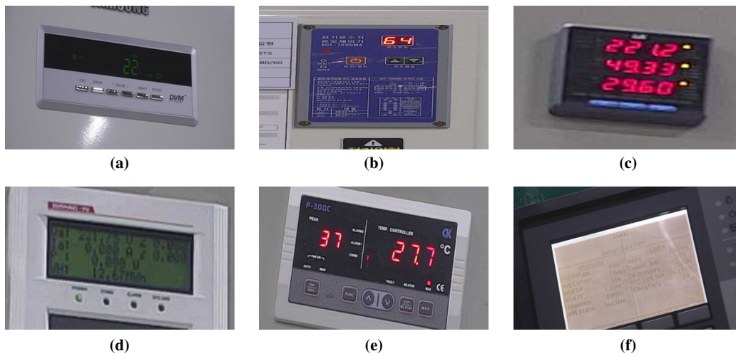
Figure 10: Digital gauge reading results of representative samples by type. (a) Air conditioner GT: 22/sVLM: 22 (b) Water heater GT: 64/sVLM: 64 (c) Pump GT: 221.2/sVLM: 221.2 (d) Integrated meter GT: 221.75/sVLM: 221.25 (e) Transformer temperature GT: 37/sVLM: 37 (f) On-site detection error GT: 38/sVLM: Unreadable.
