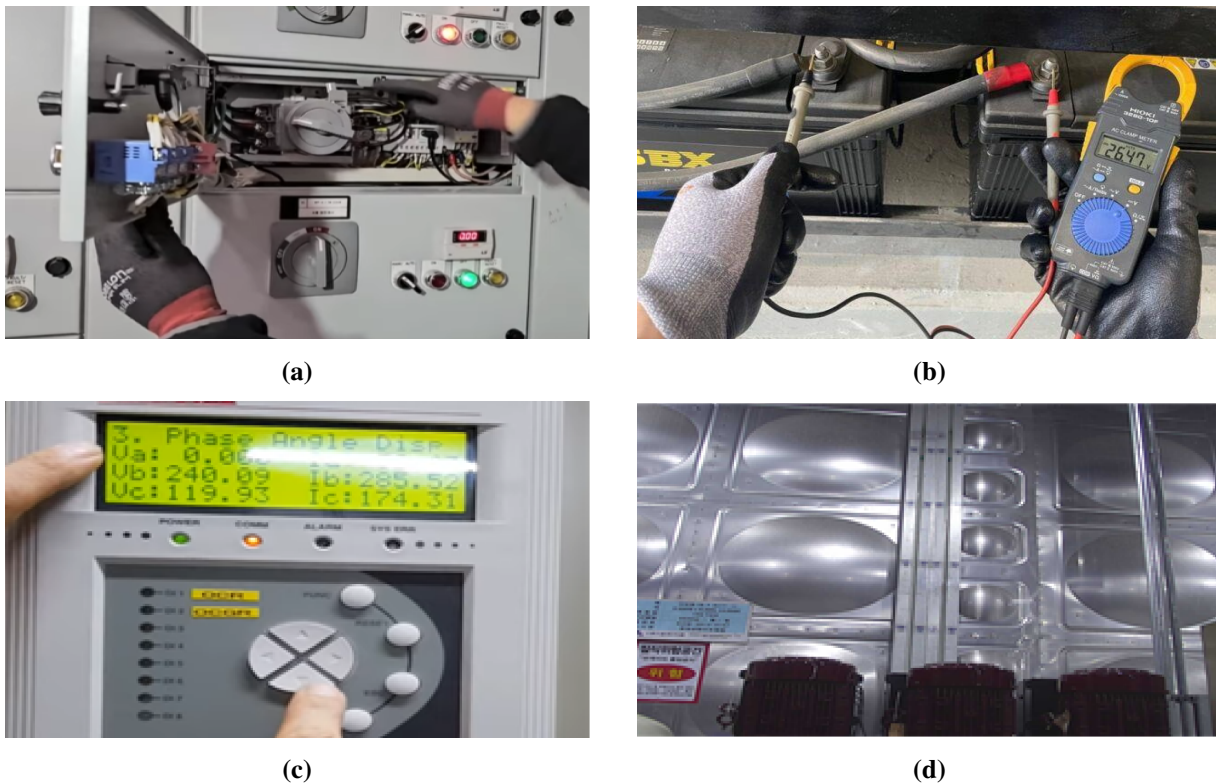
Figure 4: Key uninspectable inspection items. (a) Panel internal inspection (b) Direct measurement (c) Button operation (d) Long-range inspection.
