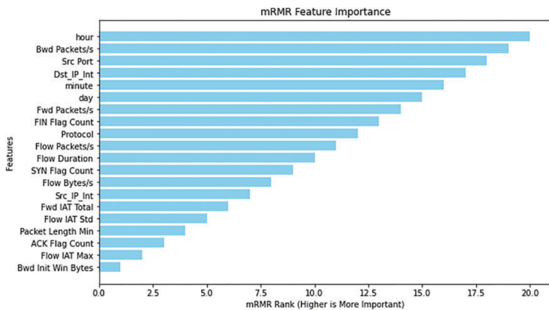
Figure 7: MRMR scores
