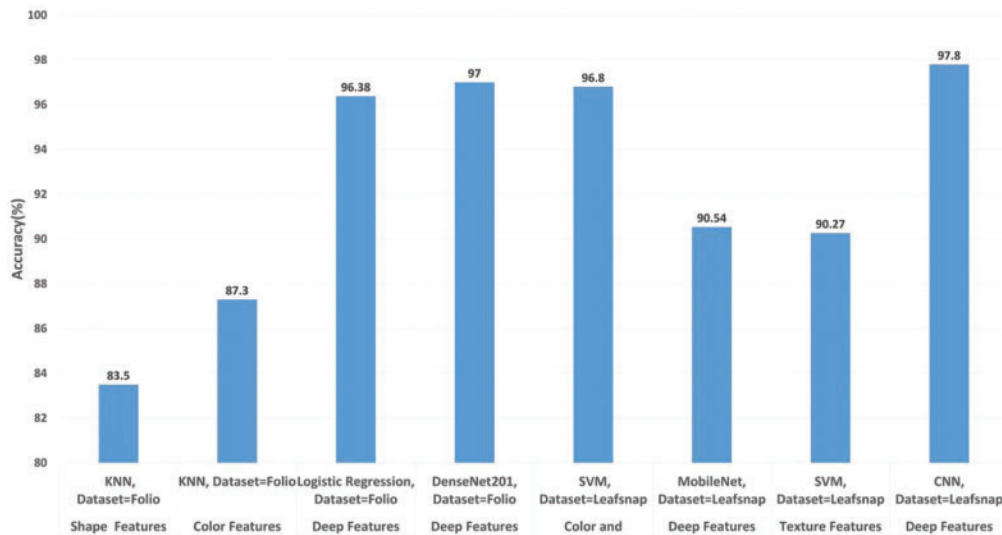
Figure 13: Studies based on leafsnap and folio datasets, employing different algorithms and features
