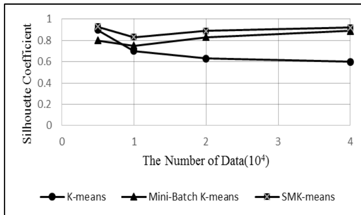
Figure 7: Comparison of the accuracy of the algorithm
