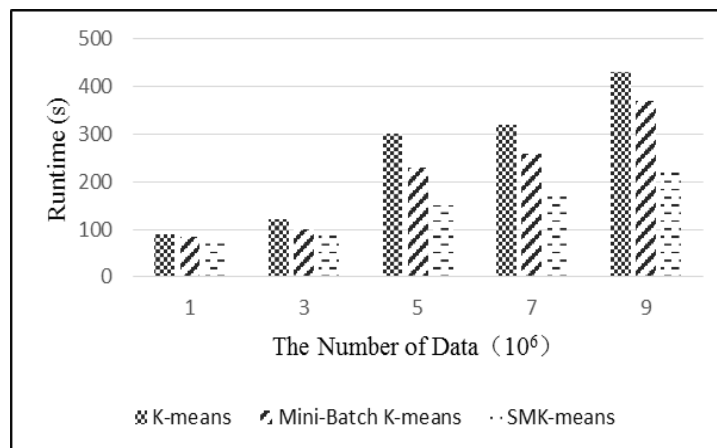
Figure 8: Algorithm runtime comparison
