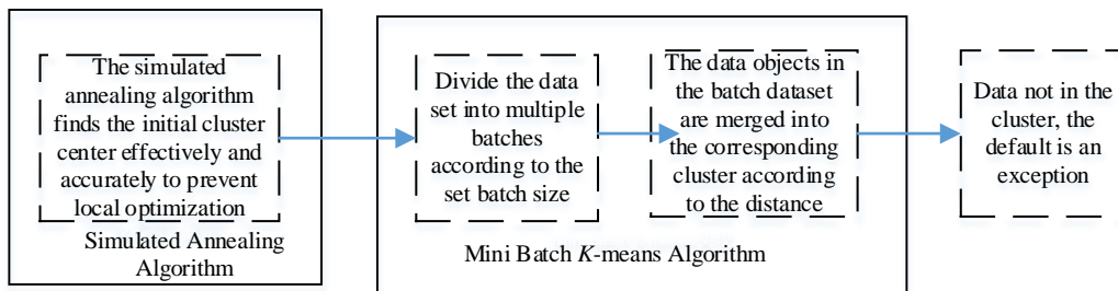
Figure 4: Parallel implementation of SMK-means algorithm
