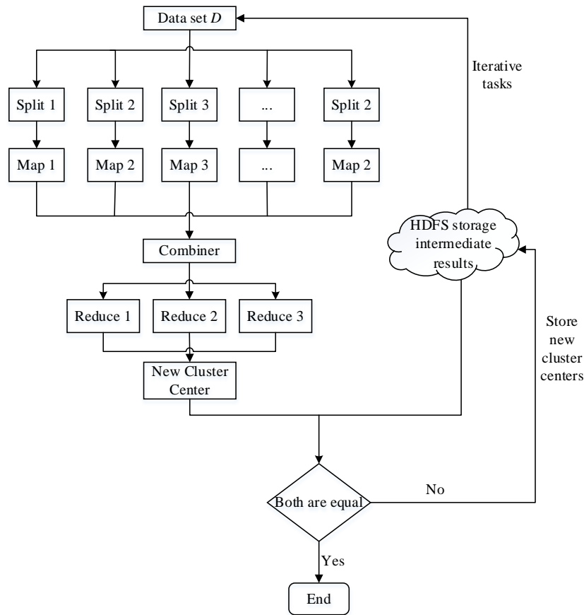
Figure 6: MapReduce parallelization flow chart of SMK-means algorithm
