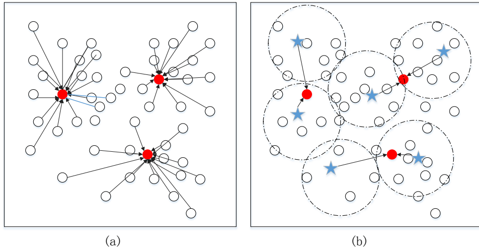
Figure 2: Two different clustering algorithm calculations: (a) K-means, (b) Mini Batch K-means
