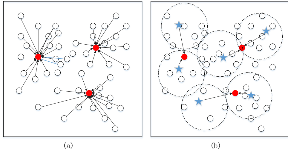
Figure 3: Two different clustering algorithms: (a) K-means algorithm; (b) Mini Batch K-means
