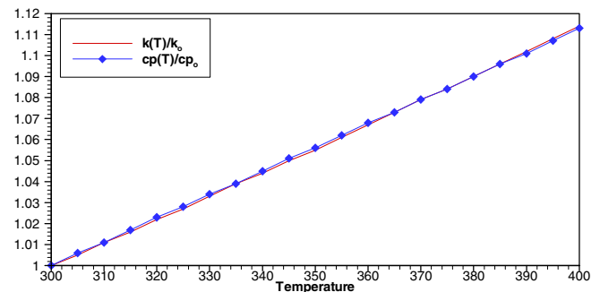
Figure 7 : Variation of the thermophysical properties for the example problem.
