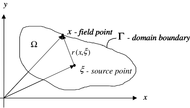
Figure 2 : Illustration of the domain \Omega bounded by the boundary \Gamma , the field point x , the source point \xi , and the r(x, \xi) is the radial distance between the field point and the source point.
