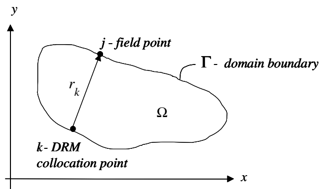
Figure 4 : Illustration of radial distance r_k used in conic RBFs.
