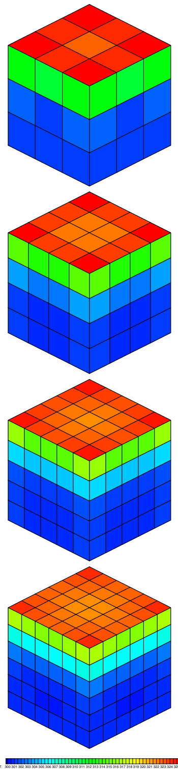
Figure 8 : Surface temperature distribution after 1 second predicted by the DRBEM using four different discretization levels.
