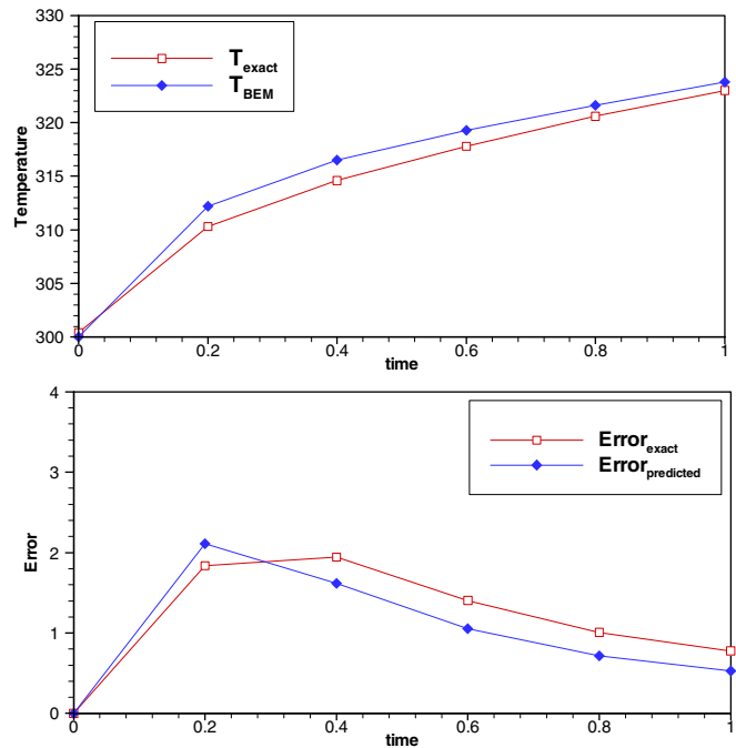
Figure 10 : Comparison of BEM and exact solutions and comparison of exact and predicted error for the 4 x 4 x 4 mesh configuration.
