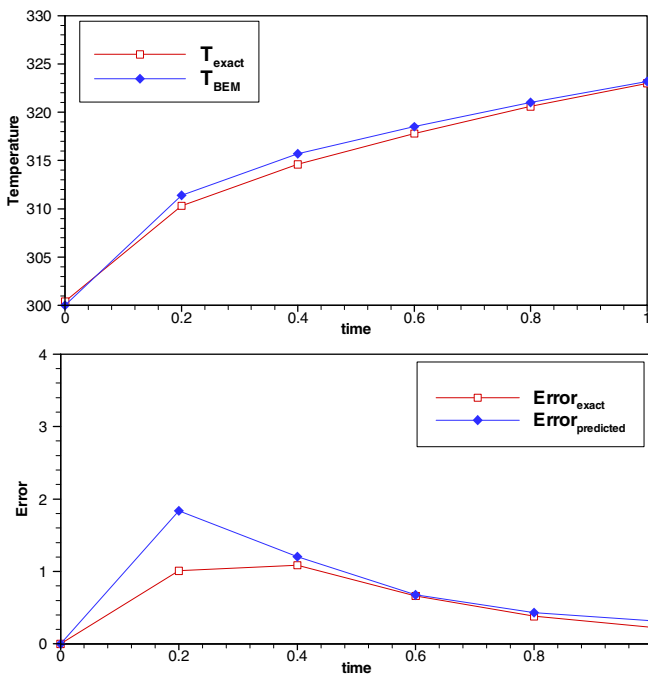
Figure 11 : Comparison of BEM and exact solutions and comparison of exact and predicted error for the 5 x 5 x 5 mesh configuration.
