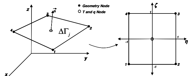
Figure 3 : Constant boundary element.
