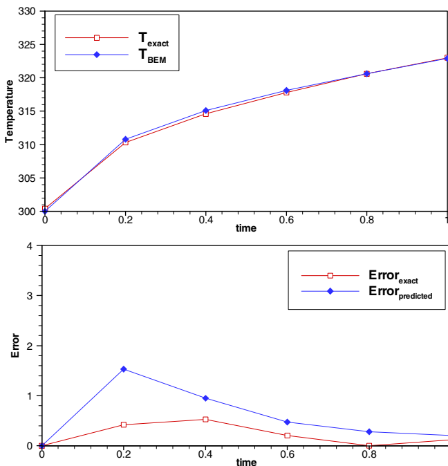
Figure 12 : Comparison of BEM and exact solutions and comparison of exact and predicted error for the 6 x 6 x 6 mesh configuration.
