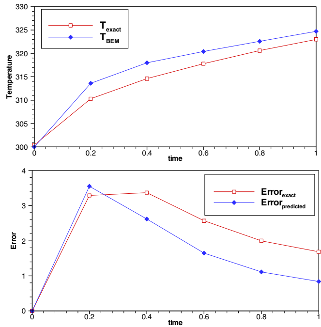
Figure 9 : Comparison of BEM and exact solutions and comparison of exact and predicted error for the 3 x 3 x 3 mesh configuration.
