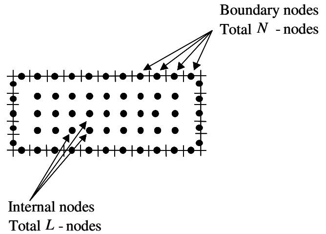
Figure 1 : Two-dimensional example of a constant element DRBEM discretization: N -boundary points corresponding to constant element nodes and L -internal points.
