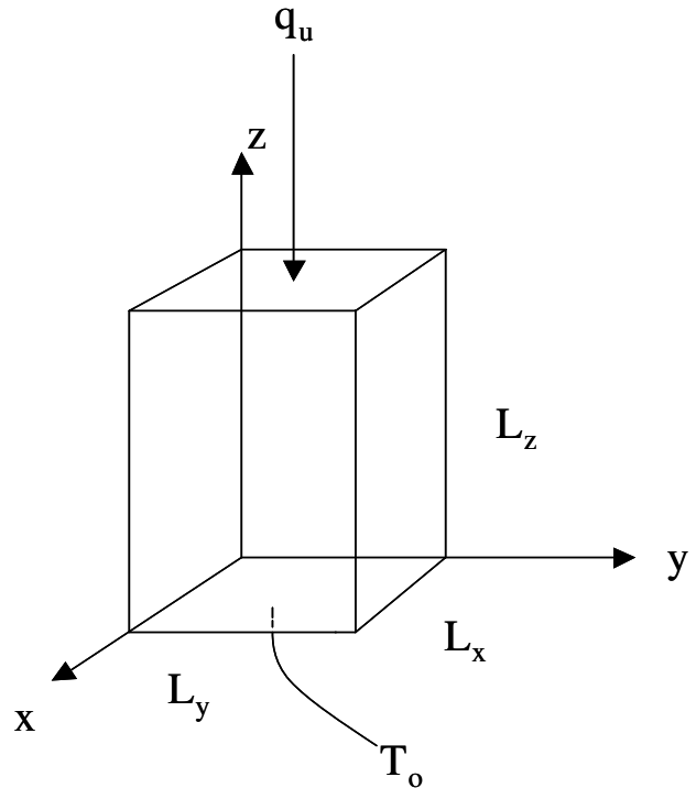
Figure 6 : Rectangular parallelepiped subjected to a constant temperature, T_o , at z = 0 , a constant heat flux, q_u , at z = L_z , and insulated on all other surfaces.
