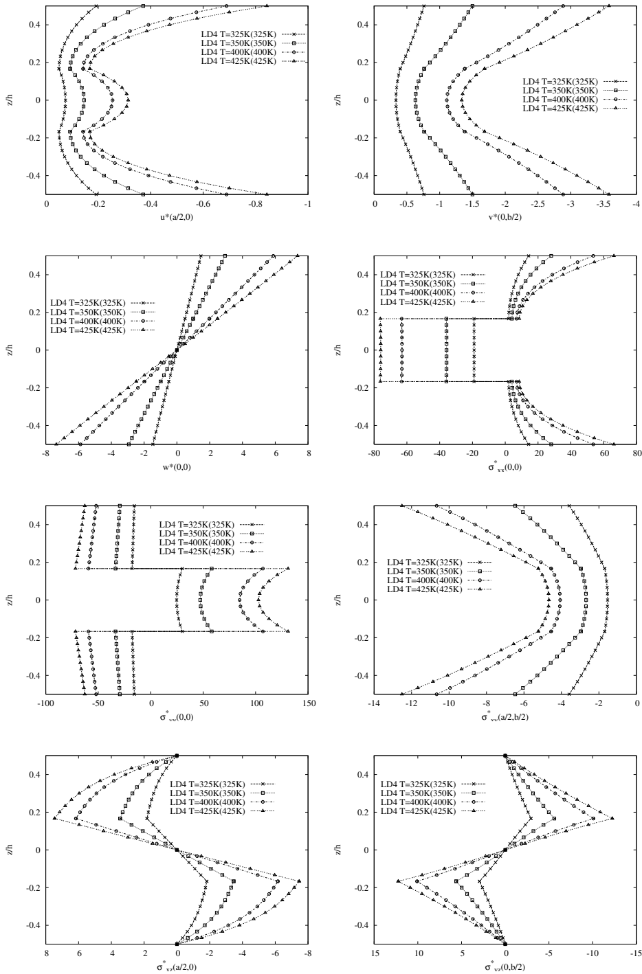
Figure 4: Second assessment: constant-through-the-thickness over-temperature \theta = T - T_0 with T = 325K, 350K, 400K, 425K and T_0 = 300K for a three-layered composite plate. LD4 model when the material properties are considered at the T value imposed.
