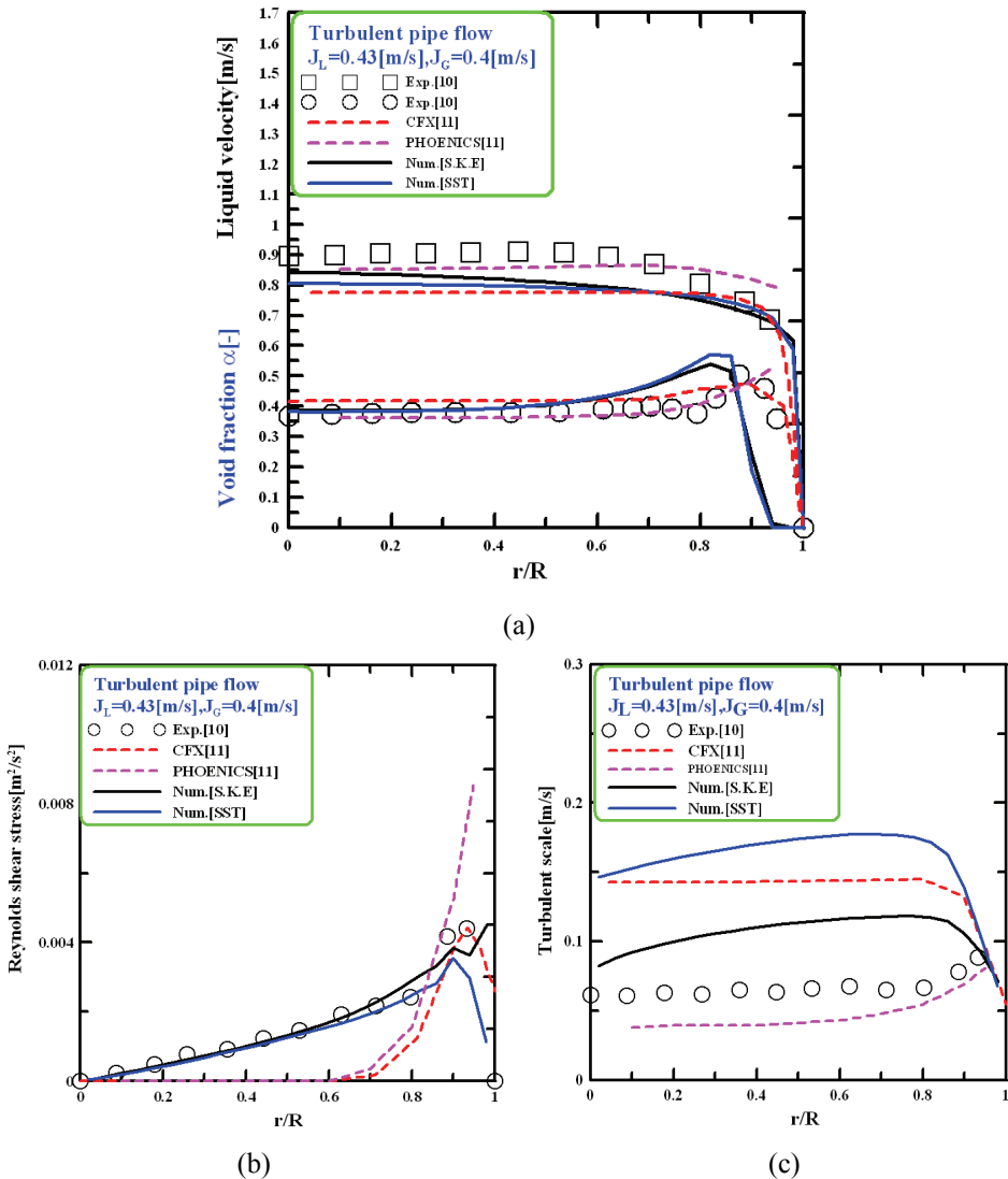
Figure 4: Verification of the present simulation via comparisons with available measurements and previous computations: Case W3 (a)Void fraction and liquid velocity, (b)Reynolds shear-stress, (c)R.M.S. liquid velocity
