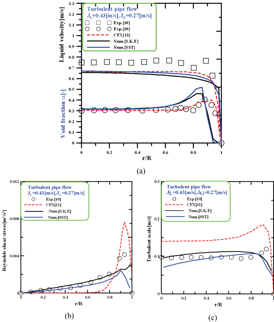
Figure 3: Verification of the present simulation via comparisons with available measurements and previous computations: Case W2 (a)Void fraction and liquid velocity, (b)Reynolds shear-stress, (c)R.M.S. liquid velocity
