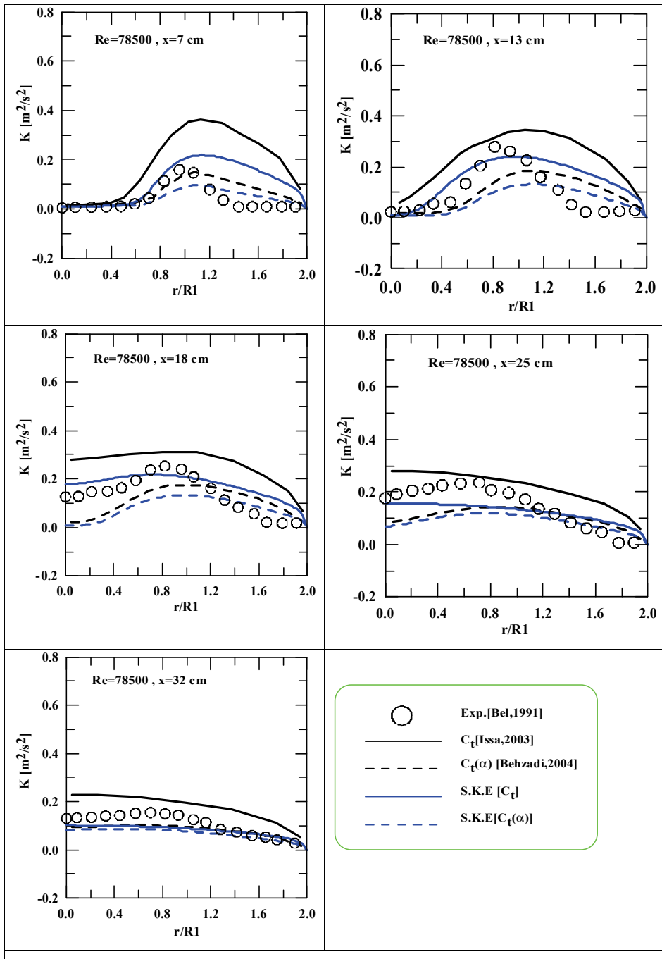
Figure 8: Turbulence kinetic energy profiles obtained from Issa and Behzadi models compared with experiment.
