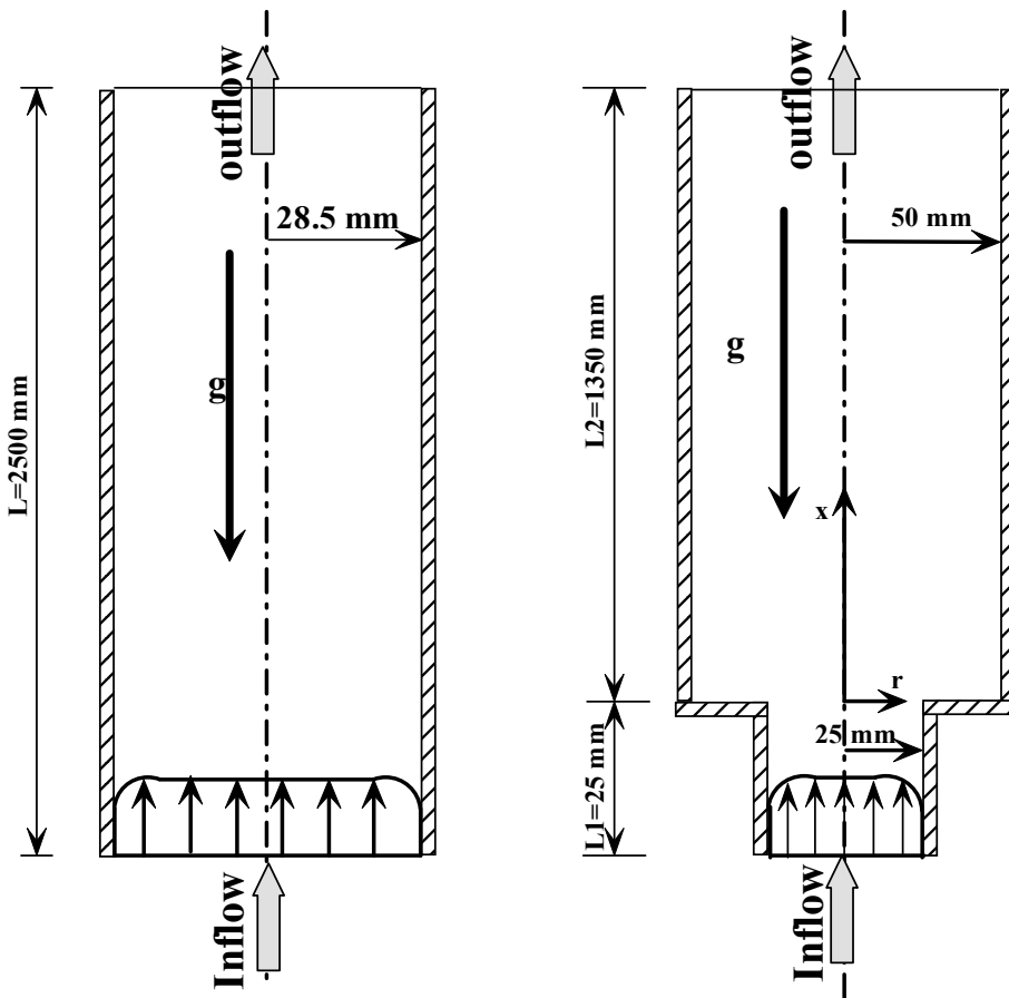
(a) Pipe flow (geometry and boundary conditions)
