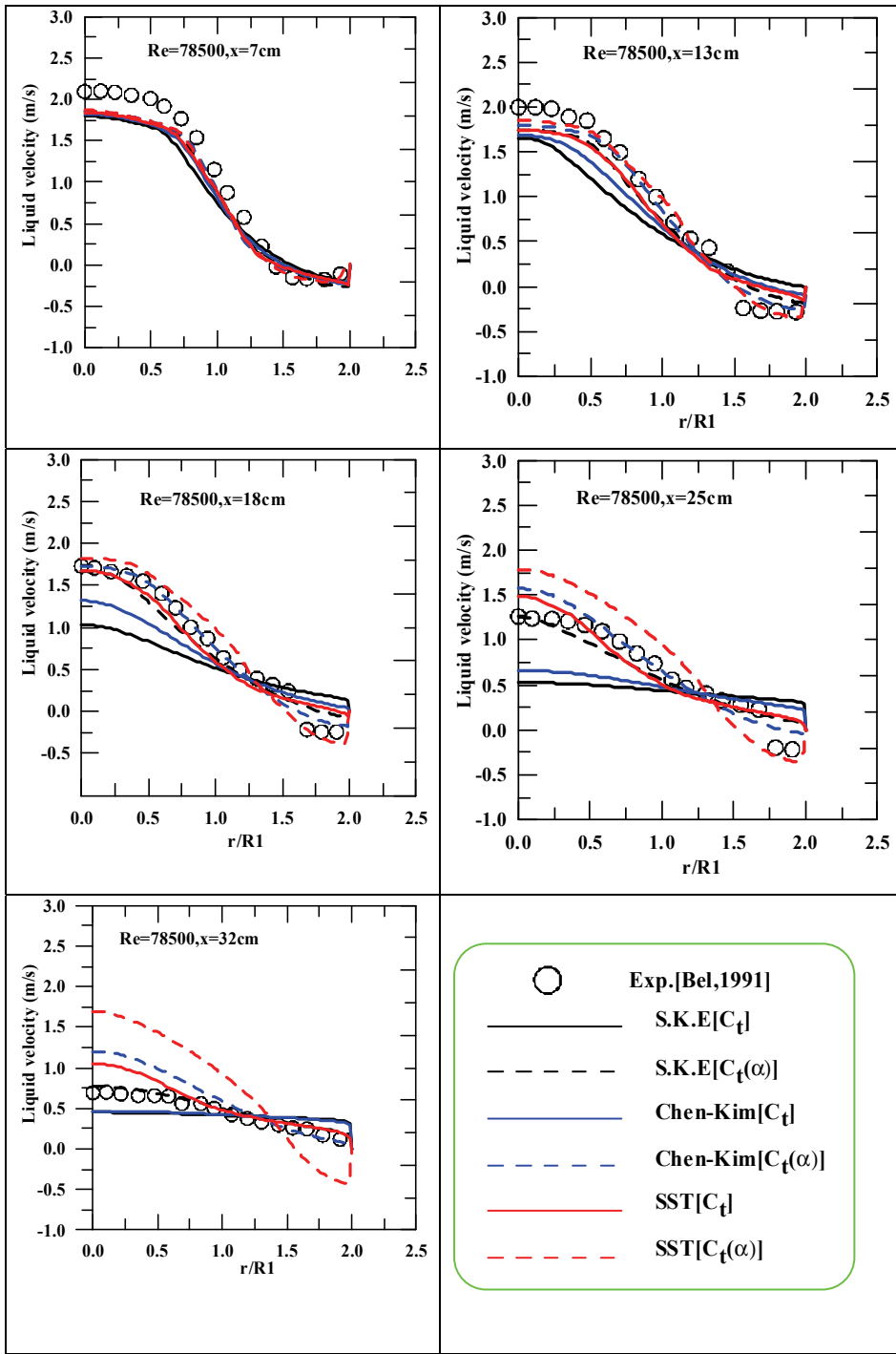
Figure 9: Continuous phase velocity profiles obtained from Issa and Behzadi models compared with experiment.
