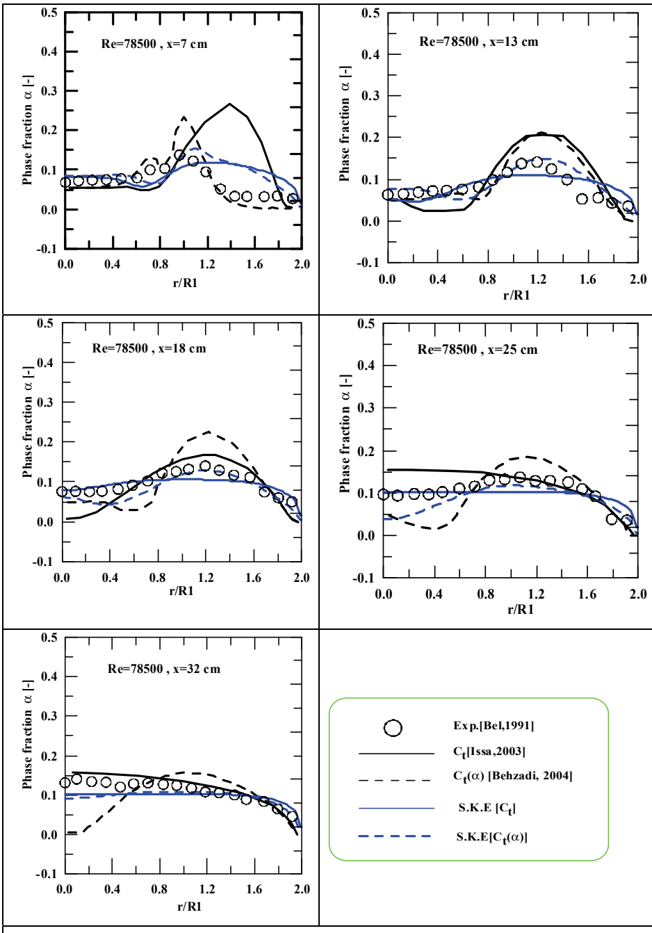
Figure 7: Phase fraction profiles obtained from Issa and Behzadi model compared with experiment.
