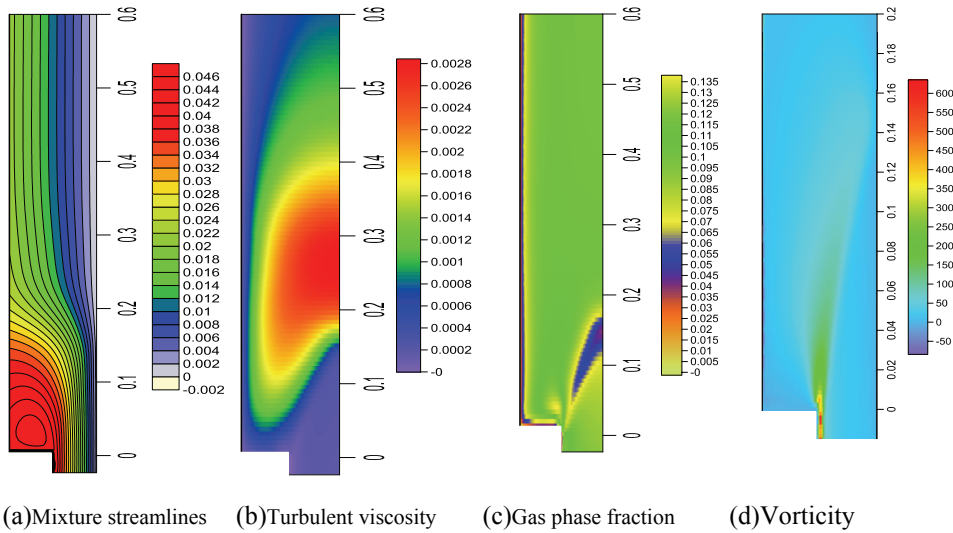
Figure 5: Prediction for the sudden expansion flow: (a) Mixture streamlines, (b) Turbulent viscosity contours, (c) Void fraction contours (d) Vorticity contours.
