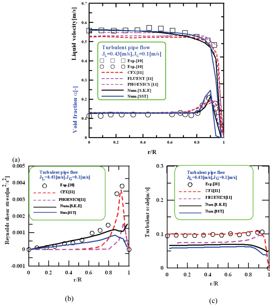
Figure 2: Verification of the present simulation via comparisons with available measurements and previous computations: Case W1 (a) Void fraction and liquid velocity, (b) Reynolds shear-stress, (c) R.M.S. liquid velocity
