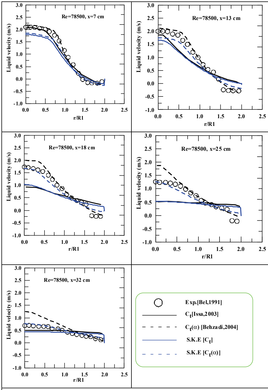
Figure 6: Continuous phase velocity profiles obtained from Issa and Behzadi model compared with experiment.
