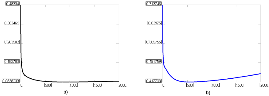
Figure 4: L_2 -errors after 2000 alternating iterations for the displacements (a) and for the tractions (b) in case of a 10% input data perturbation.
