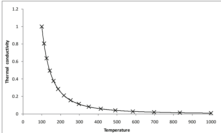
(a) Thermal conductivity k(T)
