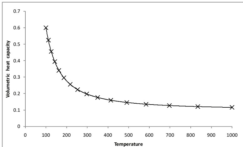
(b) Volumetric heat capacity c_v(T)
