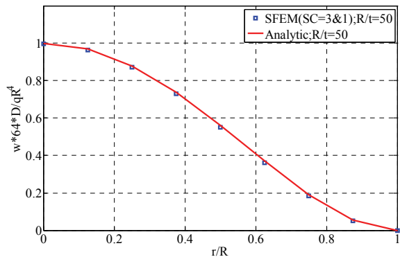
Figure 12: Deflection for the clamped circular plate subjected to uniform load along the radial line.
