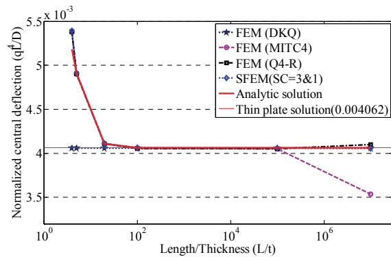
Figure 7: Shear locking test for a simply supported square plate.
