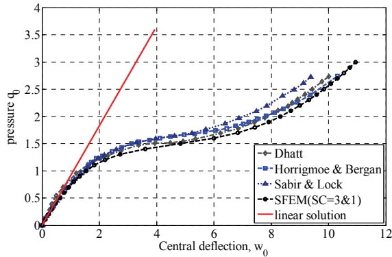
Figure 15: Nonlinear response of a clamped cylindrical shell panel to a uniformly distributed load.
