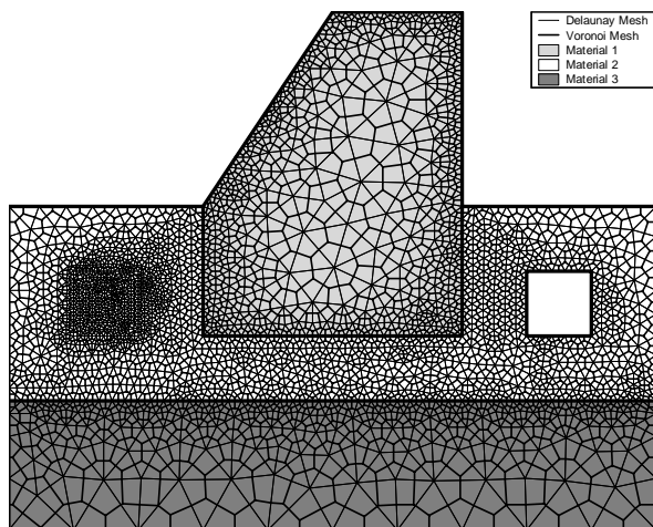
Figure 7 : Meshed Domain
