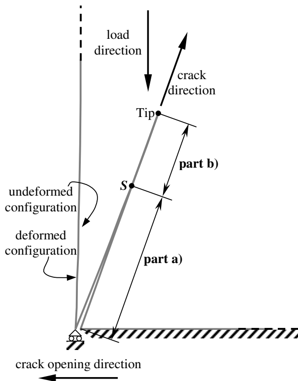
Figure 14 : Mixed-Mode crack loading
