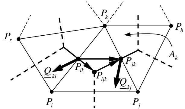
Figure 5 : Property of the stress field
