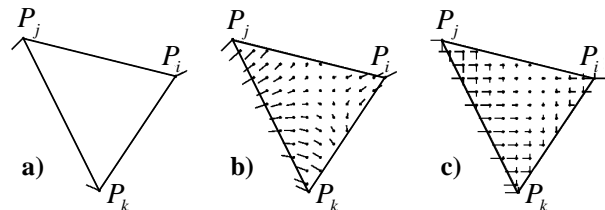
Figure 4 : Nodal displacements (a), displacement field (b), and displacement components (c) assuming an affine field
