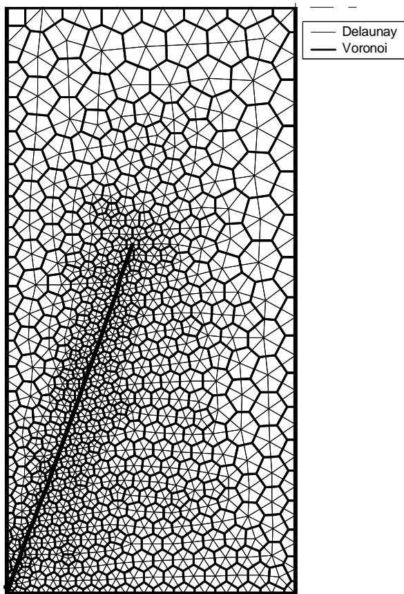
Figure 21 : Numerically predicted crack path for a compressive cylinder test
