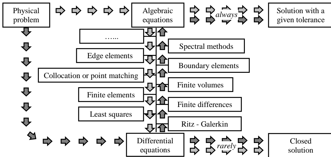
Figure 1: Comparison between the CM ( \Leftrightarrow ) and differential methods ( \Rightarrow )
