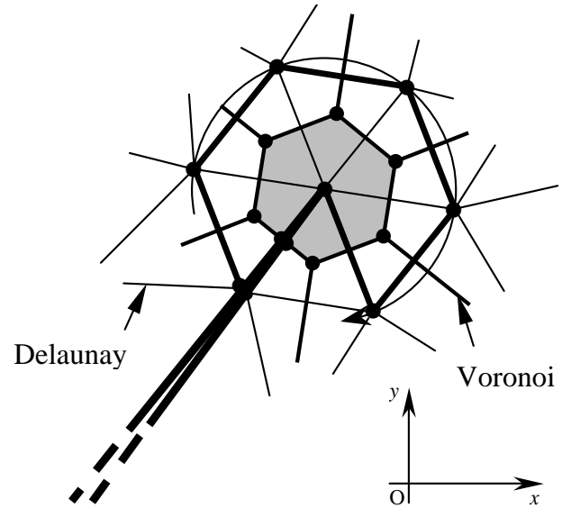
Figure 8 : First hexagonal kernel at the crack tip
