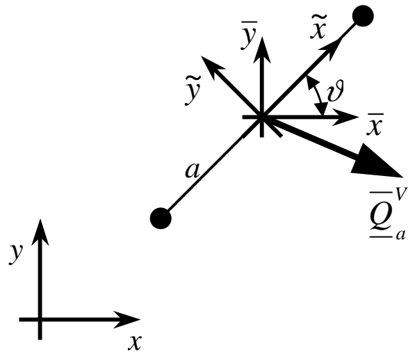
Figure 10 : Global and local reference frames for a Voronoi side a
