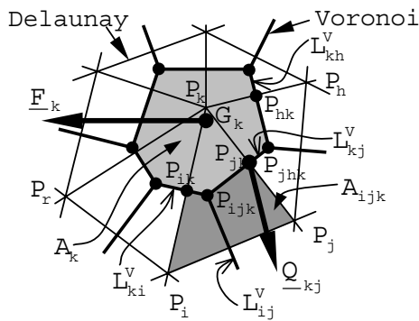
Figure 2 : The Delaunay/Voronoi mesh and the association of Voronoi geometric elements with the source variables
