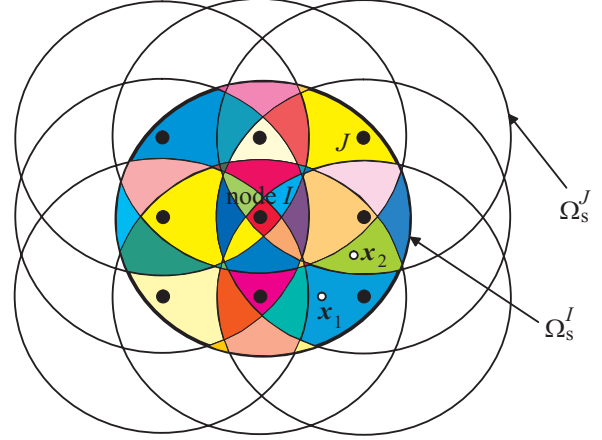
Figure 4 : The nodal shape function \phi^l(\mathbf{x}) , from the MLS interpolation, which is nonzero in \Omega_s^l , and which has a different form in each small intersection, as divided by several circular sub-domains.
