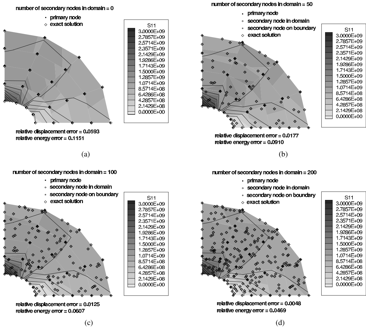
Figure 20 : Comparison of the MLPG and the exact solutions, for the problem of a plate with a circular hole. Displacements and distribution of stress \sigma_{11} (a) without secondary nodes, (b) with 50 secondary nodes, (c) with 100 secondary nodes, and (d) with 200 secondary nodes in the domain.
