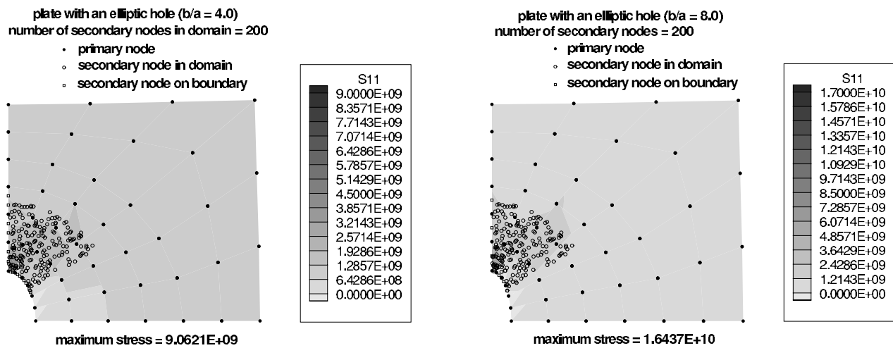
Figure 22 : The MLPG solutions for the problem of a plate with an elliptical hole: ( b/a = 4.0 and b/a = 8.0 ). Displacements and distribution of stress \sigma_{11} (a) without secondary nodes, (b) with 25 secondary nodes, (c) with 50 secondary nodes, (d) with 100 secondary nodes, and (e) with 200 secondary nodes in the domain.
