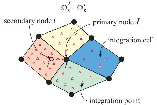
Figure 16 : Numerical integration inside each integration cell in the sub-domain \Omega_s^I = \Omega_s^i .
