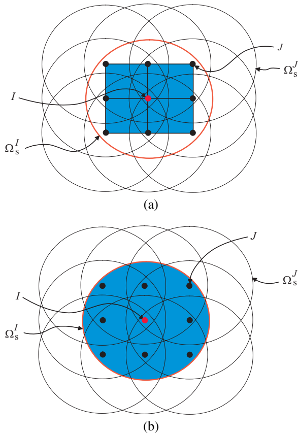
Figure 5 : Integration methods in meshless methods: (a) using background cell and (b) integration over sub-domain \Omega_s^I for node I .
