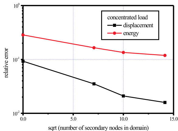
Figure 25 : Convergence for the displacement and the energy norms in the problem of a concentrated load on a semi-infinite plate, with irregularly distributed secondary nodes in the domain.
