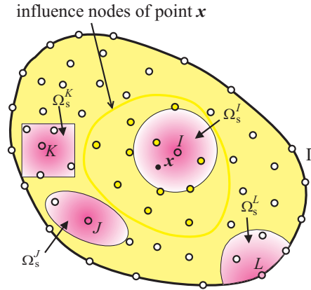
Figure 2 : A schematic illustrating various shapes for sub-domains, and the region bounding all the nodes in \Omega which may influence the interpolation at a generic x in a meshless approximation.
