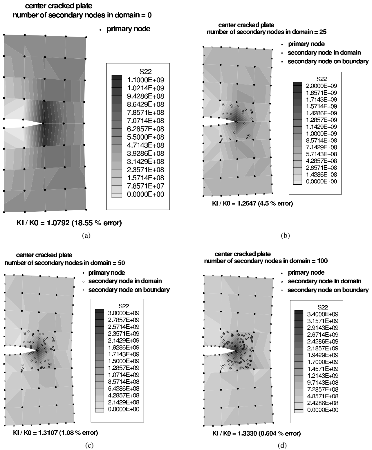
Figure 26 : The MLPG solutions for the problem of a center cracked plate. Displacements and distribution of stress \sigma_{22} (a) without secondary nodes, (b) with 25 secondary nodes, (c) with 50 secondary nodes, and (d) with 100 secondary nodes in the domain.
