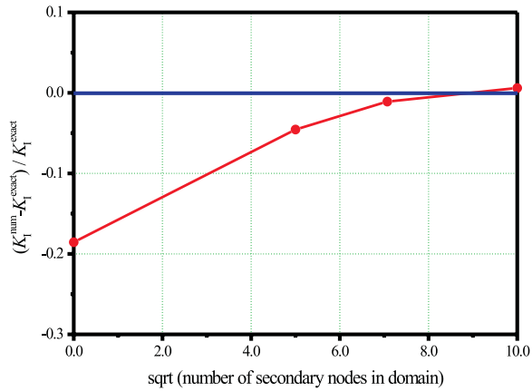
Figure 28 : Errors in the evaluation of stress intensity factor, versus the number of secondary nodes in the domain for a center cracked plate problem.
